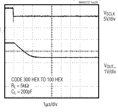
DIGITAL-TO-ANALOG GLITCH IMPULSE (VDD = +5V)
