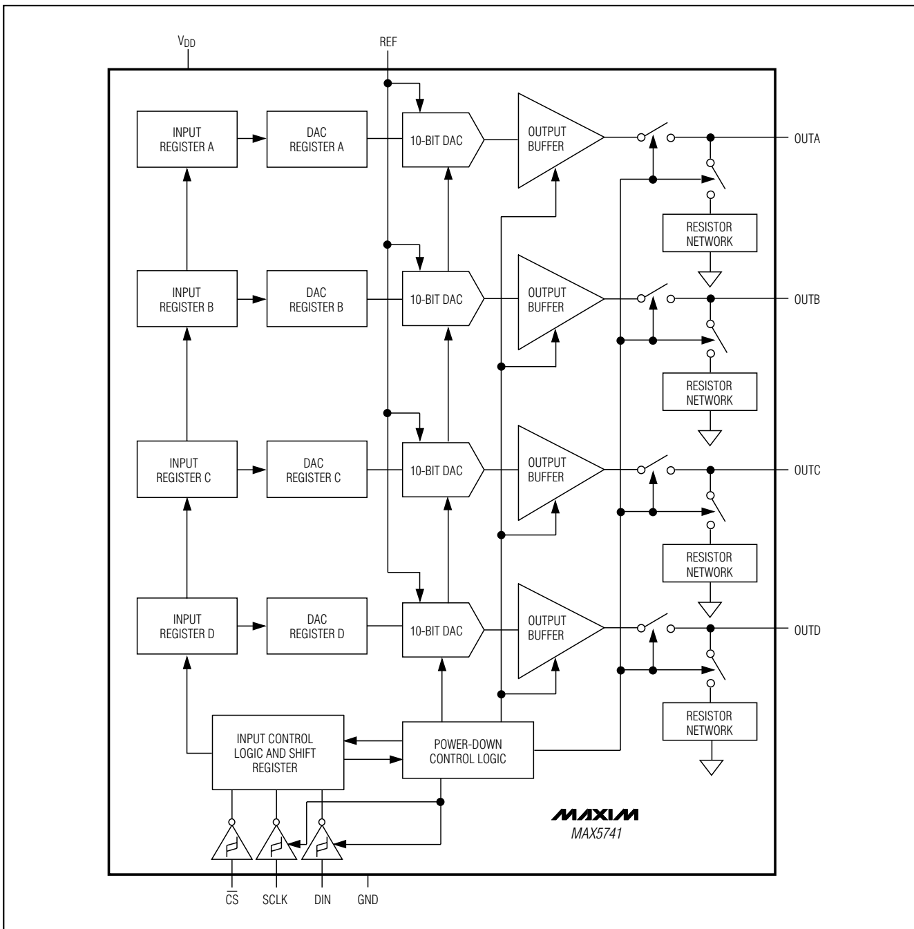
Functional Diagram
