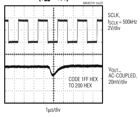
DIGITAL-TO-ANALOG GLITCH IMPULSE (VDD = +5V)
