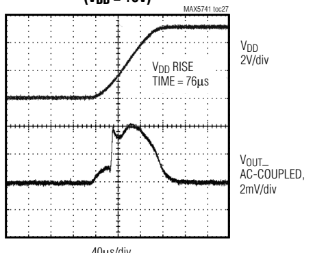
POWER-ON RESET, SLOW RISE TIME ( V_{DD} = +5\text{V} )
